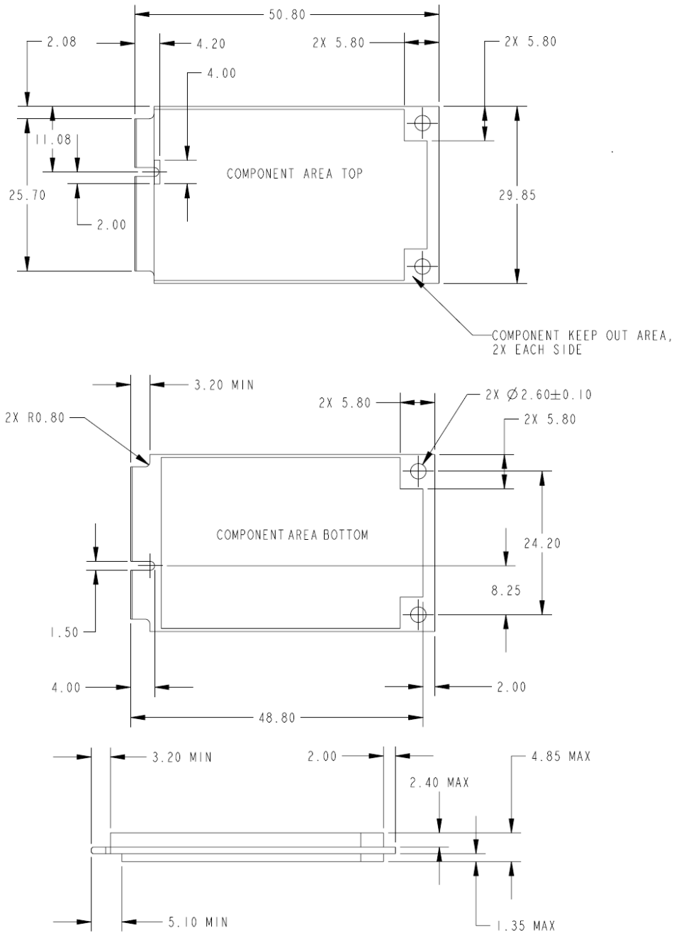
Figure 3-1: Dimensions
