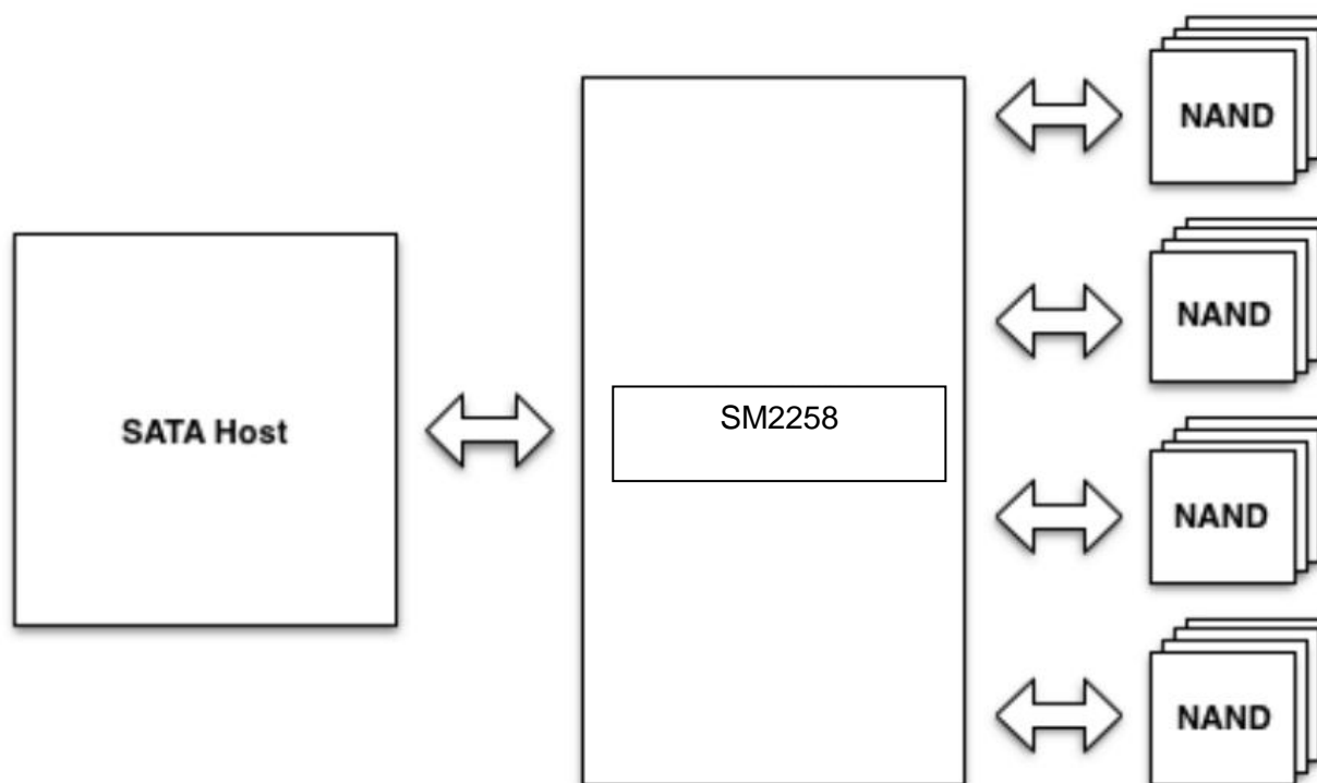
Figure 4-1: Block Diagram
