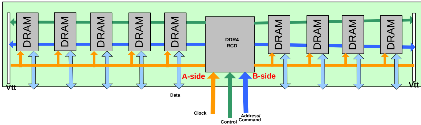
BLOCK DIAGRAM, SINGLE RANK
