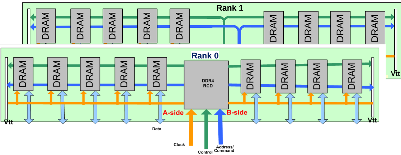
BLOCK DIAGRAM, DUAL RANK
