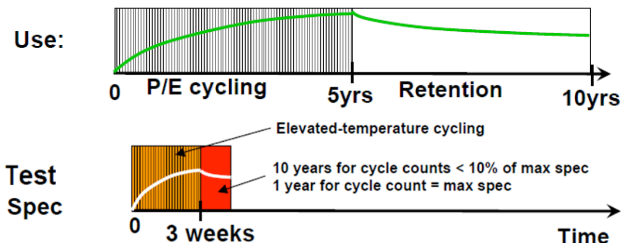
Figure 3-1: JEDEC Data Retention Test Spec
