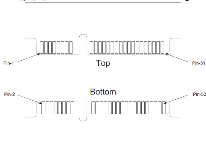
Figure 9-1: mSATA connector
