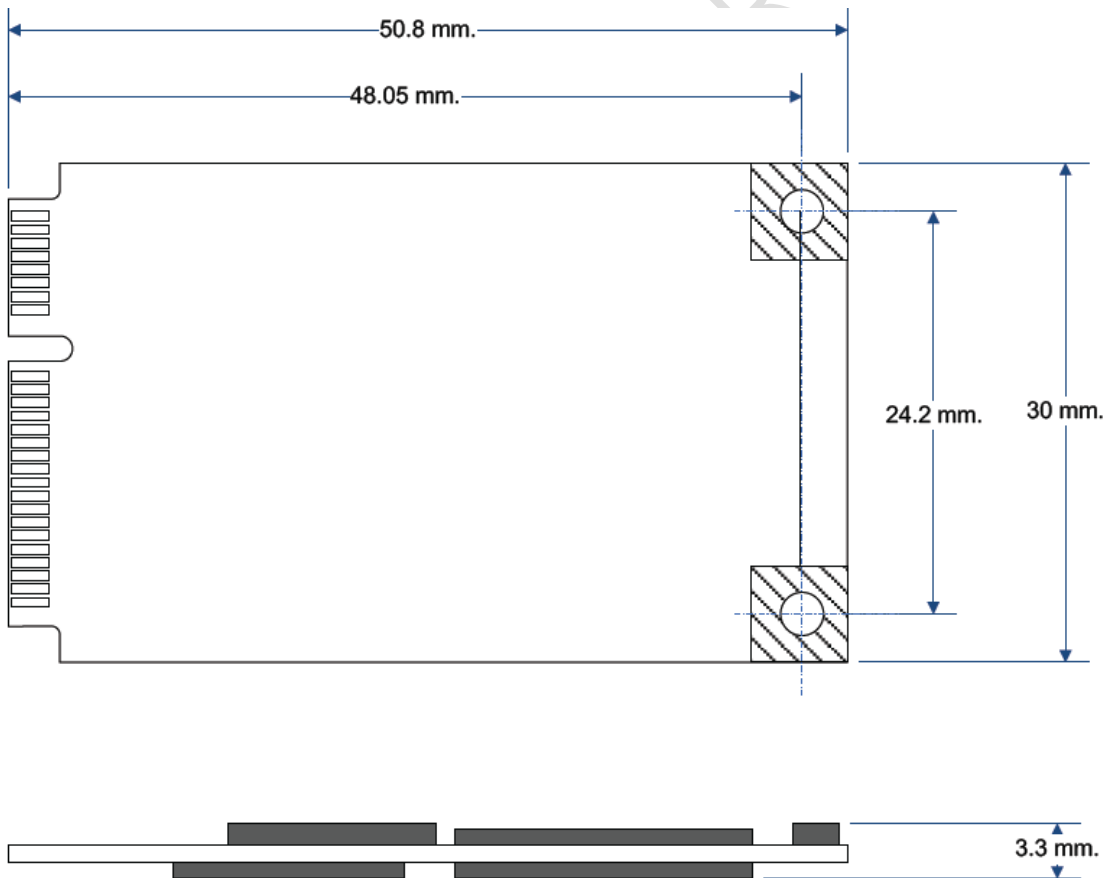
Figure 3-2: Dimension Details for MO-300 mSATA SSD
